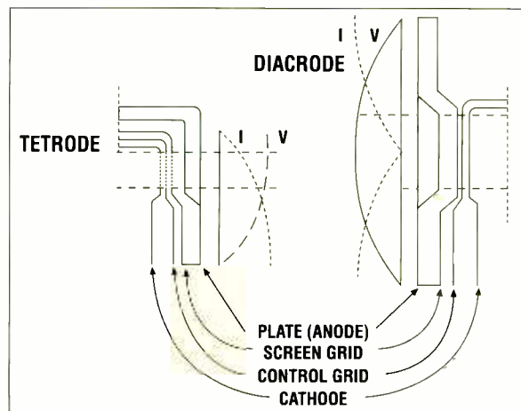
Figure 2. Cutaway view of the tetrode (left) and the Diacode (right). Note that the RF current peaks above and below the Diacode center, while on the tetrode there is only one peak at the bottom.
