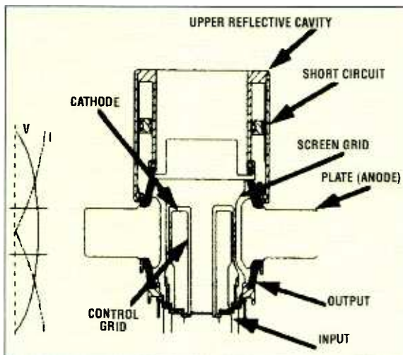
Figure 3. The elements of the Diacode, including the upper cavity. Double current, and consequently, double power, is achieved with the device because of the current peaks at the top and bottom of the tube, as shown.
