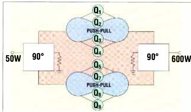
Figure 1. Diagram of a 600W VHF amplifier using eight FETs in a parallel device/parallel module configuration.
